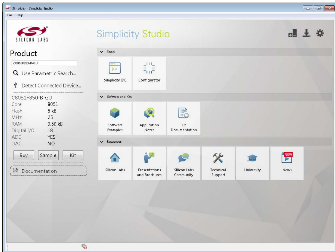
Figure 2. Simplicity Studio
