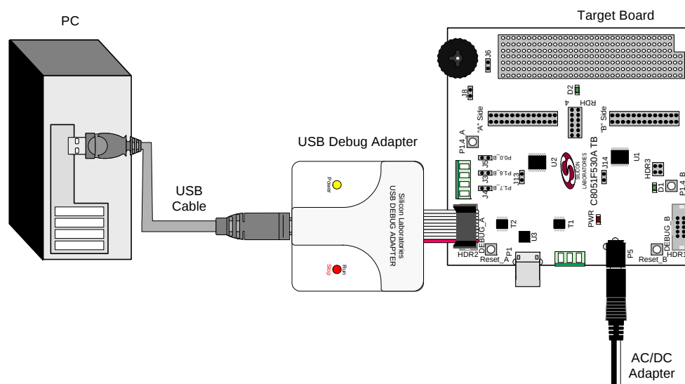
Figure 1. Hardware Setup using a USB Debug Adapter
